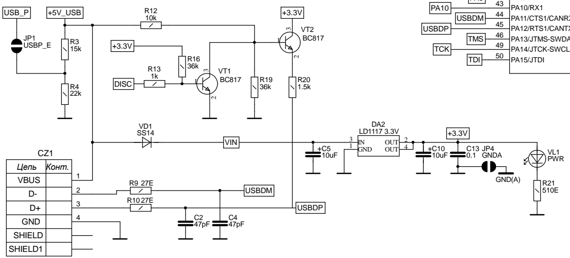
STM32F103_HB header board
