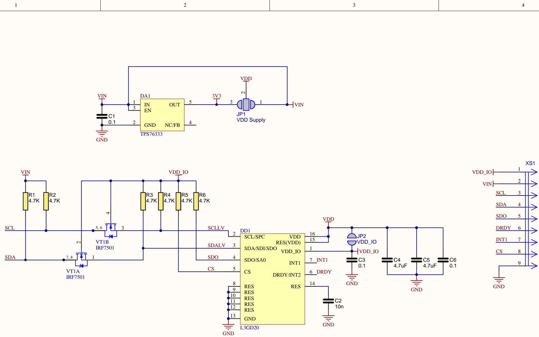
L3GD20 three-axis angular rate sensor
